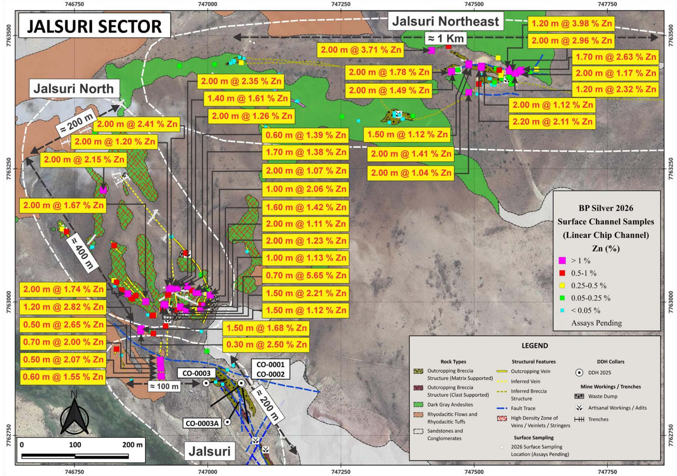
Zinc Grades From Channel Samples at Jalsuri, Jalsuri North, and Jalsuri Northeast Targets
